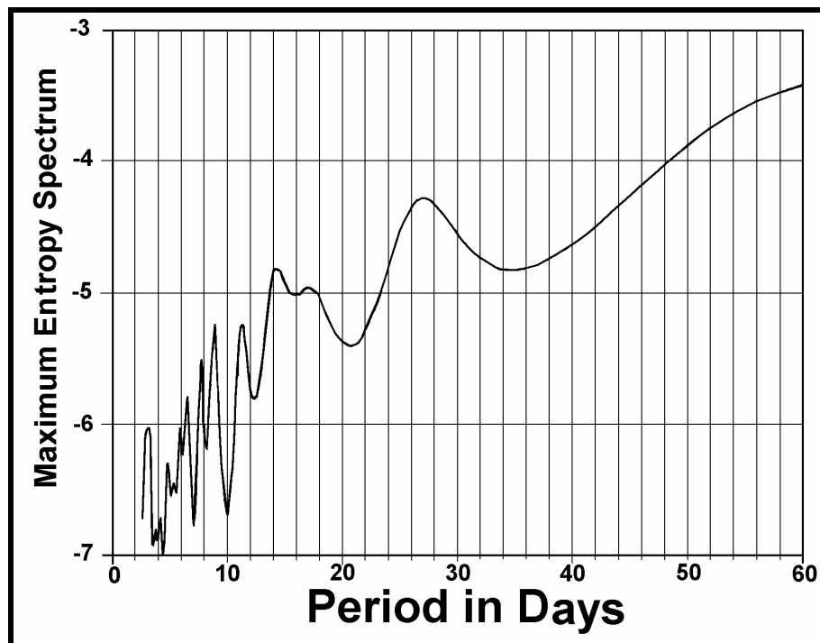
Figure 10: Maximum entropy spectrum for the 2-day average 0-20 Hz Schumann Resonance Intensity for the period February 1997 to December 1999.
