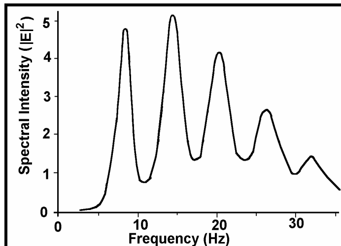
Figure 1: A typical daytime spectrum for the vertical electric field measured near Kingston, Rhode Island, showing the first five Schumann Resonances modes, Polk (1982).
