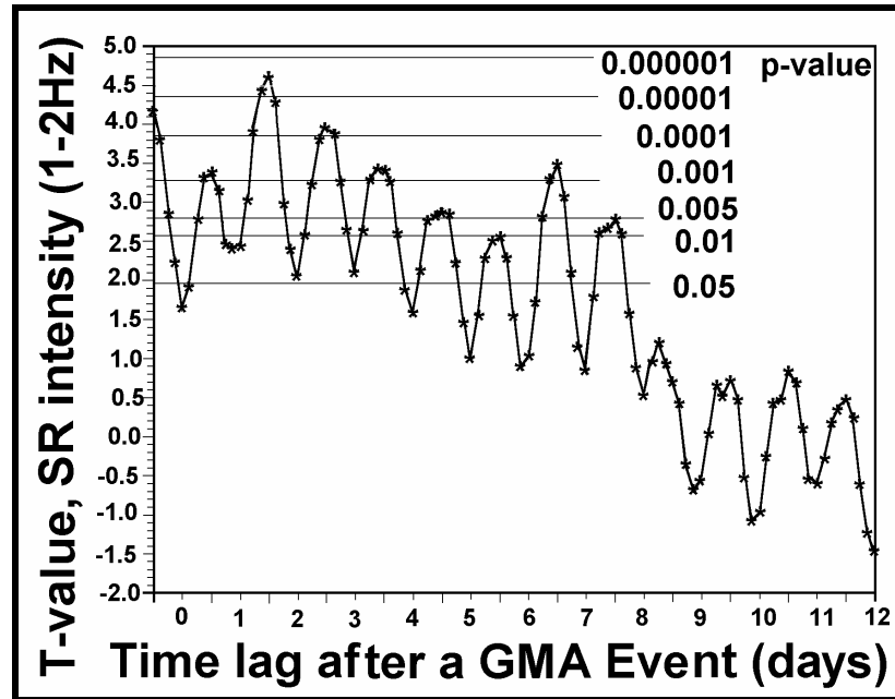
Figure 6: The statistical Student T-value of the time lagged correlation between the 3-hour Kp index and the 3-hr mean Schumann Resonance Intensity for the 1-2 Hz band, for the period September 1996 to December 1999.
