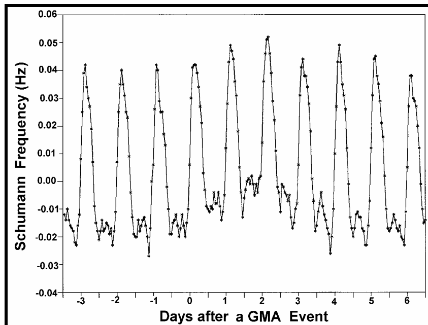
Figure 8: Superimposed epoch analysis of the impact of a Geomagnetic events, as defined by the Kp Index, for the Schumann Resonance 8Hz band frequency anomaly for 69 events in 1997 to 1999.
