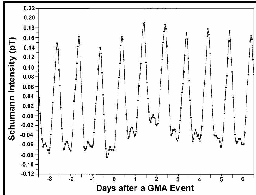
Figure 7: Superimposed epoch analysis of the impact of a Geomagnetic events, as defined by the Kp Index, for the mean anomaly in the Schumann Resonance 0-20 Hz intensity for 69 events in 1997 to 1999. GMA events occurred on day zero.
