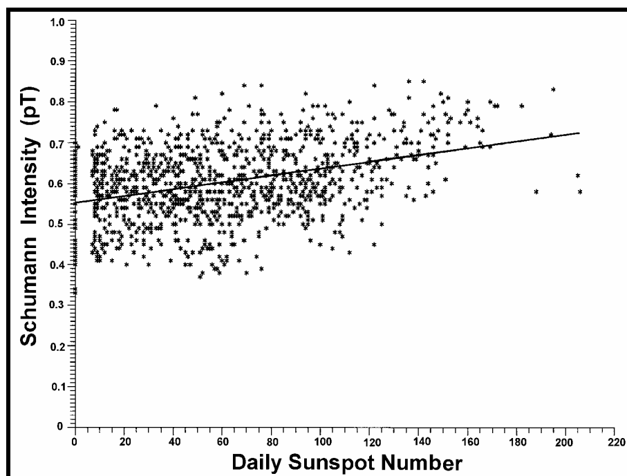
Figure 9: Daily mean SR intensity (0-20Hz) as a function of daily sunspot number for the period 12/1/97 to 31/12/99.
