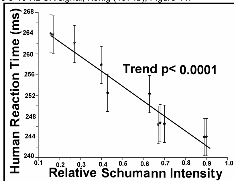
Figure 11: Human reaction times as a function of Schumann Resonance 8-10 Hz relative intensity. Reaction times measured using a light flash and a Morse key, tested during 18 days in September 1953, at the German Traffic exhibition in Munich. Each point represents 4500 subjects, with the mean variance of 3.6 ms shown as error bars. Trend: t = 10.414 , 2-tailed p < 0.0001 . Data is derived from Figure 3 of König (1974b). The relative intensity is estimated to be in the range 0.6 to 1 pT for the 0-20 Hz band.
